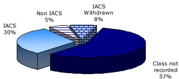
Graph 61 - World fleet : total number of 25+ years old ships, by class - 2005
