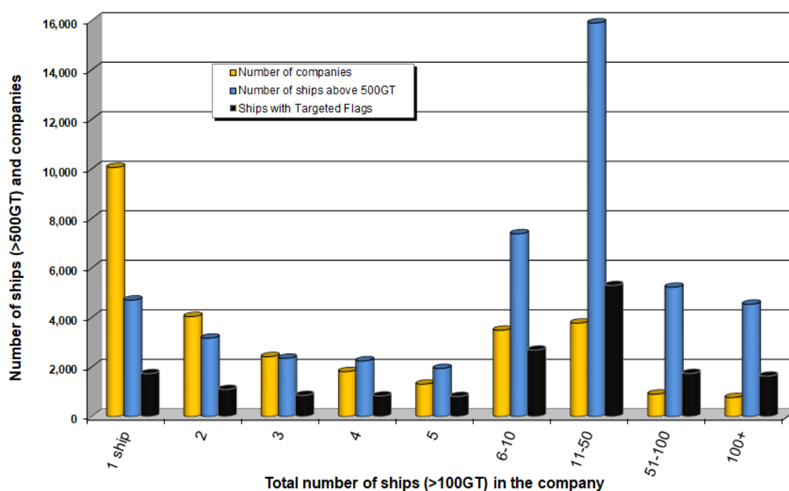
Graph 139 -Total number of companies and ships GT \geq 500, by company fleet size
